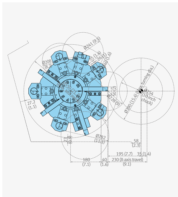
PUMA GT2100B (2axis, 10station)
