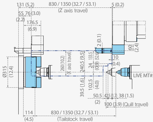
ID Holder
