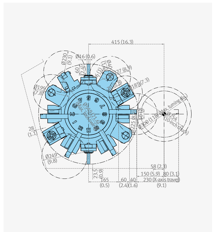
PUMA GT2100MB (M, 12station, BMT55P)
